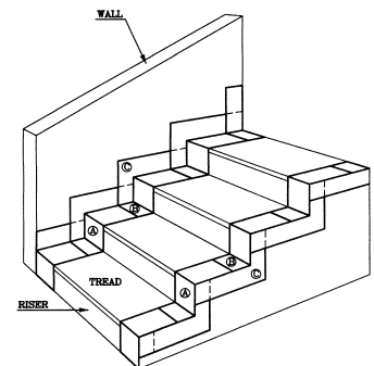
90.7 Sheet Metals (Flashing) for Stairs
