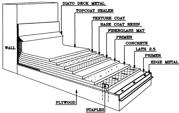
1.1 AVM System 100 - Elasto Fiberdeck® Over Plywood Substrate
