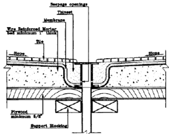
AVM System 700, Under Tile or Shower Drain
