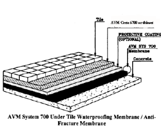
FIGURE 1—TYPICAL INSTALLATION DETAILS
