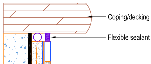
Alternate deck profile
