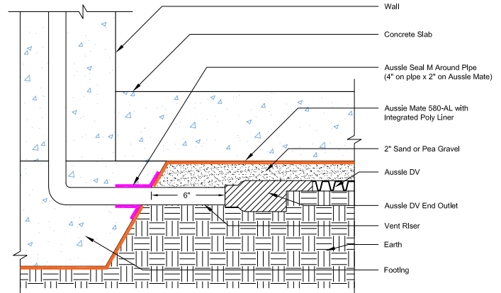
FIGURE 4.6 - DV CONNECTION
