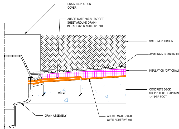
FIGURE 3.4 - DECK DRAIN WITH INSPECTION COVER
