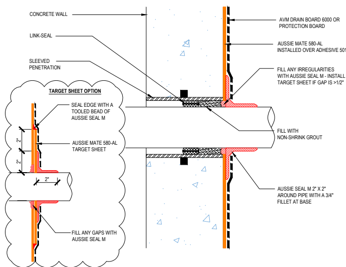
FIGURE 2.3 - SLEEVED PIPE PENETRATION
