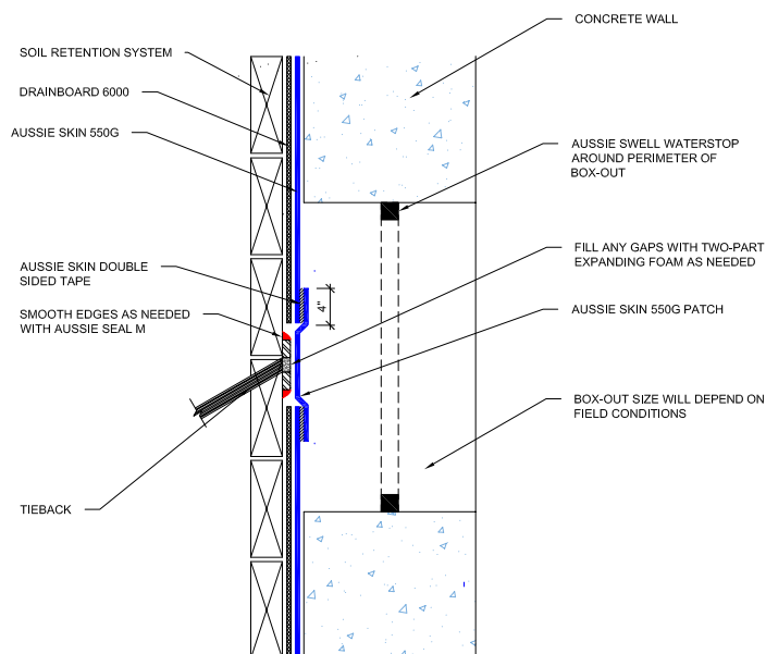
FIGURE 2.7 - SLEEVED PIPE PENETRATION PROPERTYLINE
