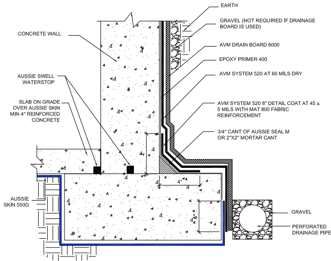
FIGURE 1.9 - AUSSIE SKIN UNDER SLAB TIED INTO AVM SYSTEM 520 UP WALLS.
