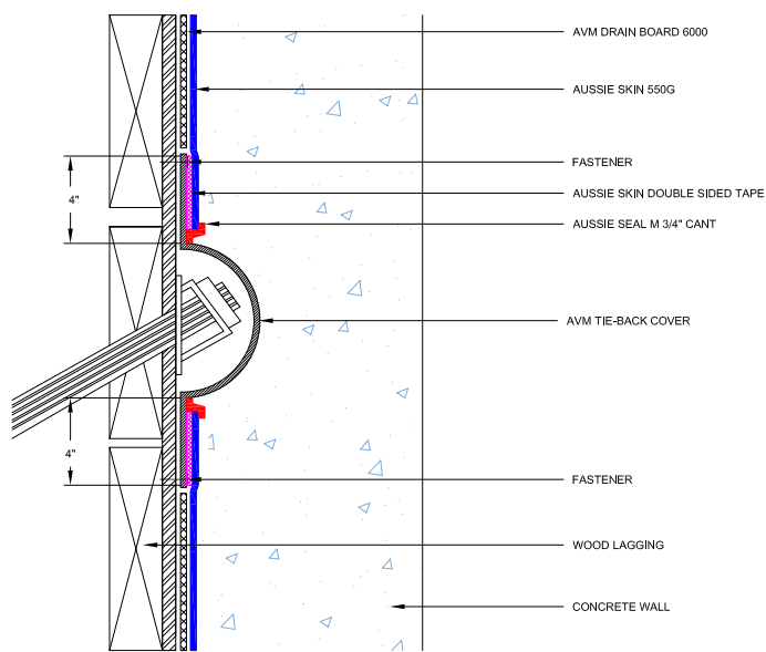
FIGURE 2.6 - TIE-BACK COVER DETAIL
