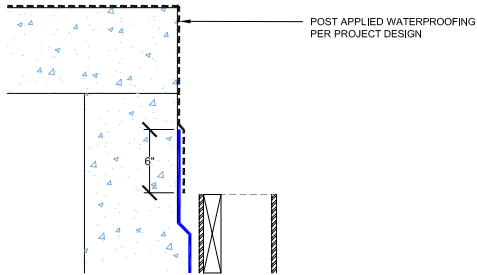
FIGURE 2.12 - LAGGING BOARD REMOVAL AT GRADE
