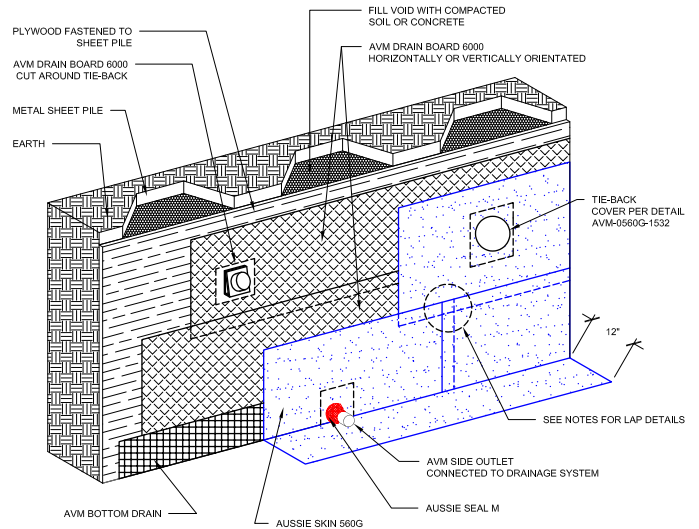
FIGURE 1.17 - SHEET METAL PILING
