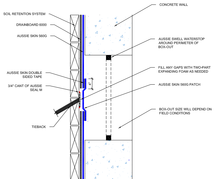
FIGURE 2.8 - DE-TENSIONING OF TIE BACK W/ BOX OUT
