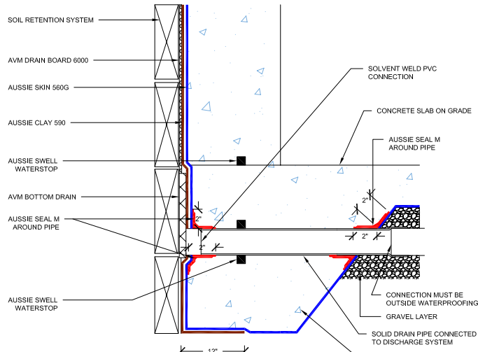
FIGURE 3.3 - NON-HYDROSTATIC RAISED SLAB
