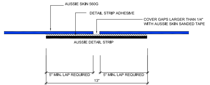
FIGURE 1.6 - NON-FACTORY LAP WITH DETAIL STRIP
