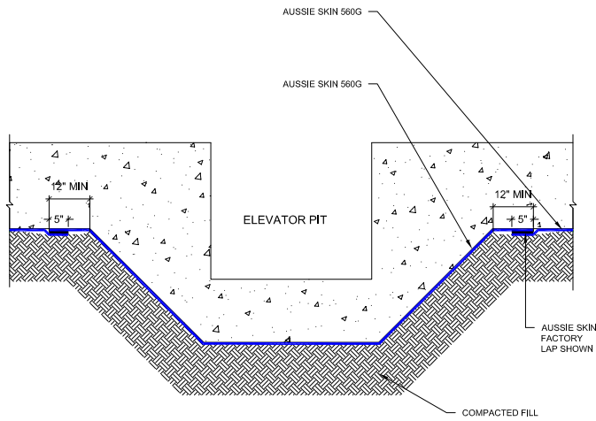
FIGURE 1.15 - ELEVATOR PIT
