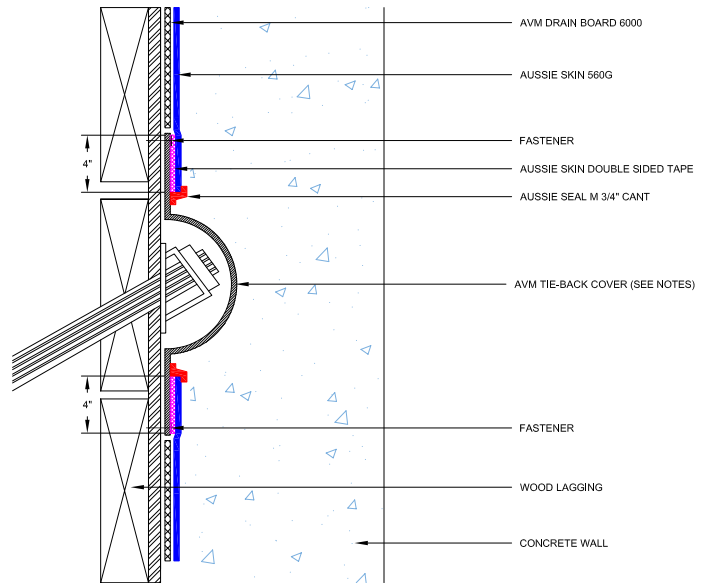
FIGURE 2.7 - TIE BACK COVER DETAIL
