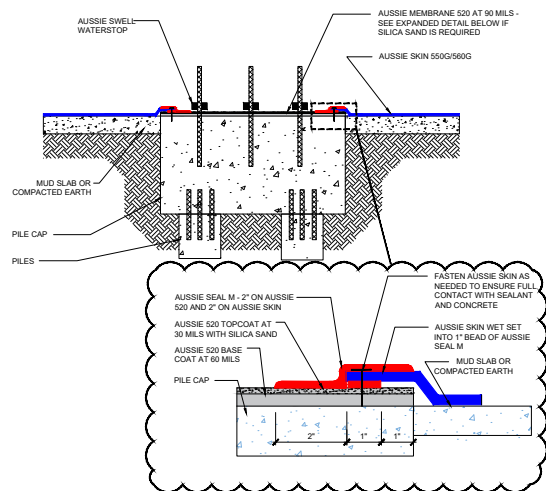
FIGURE 1.14 - HYDROSTATIC PILE CAP WITH AUSSIE SKIN 560G
