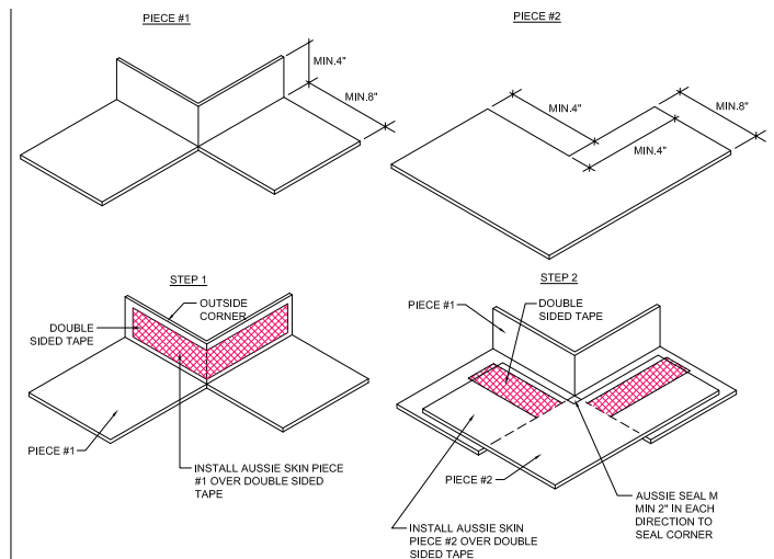
FIGURE 1.19 - OUTSIDE CORNER
