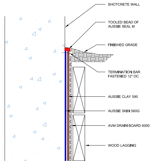
FIGURE 3.10 - GRADE TERMINATION OPTION 1
