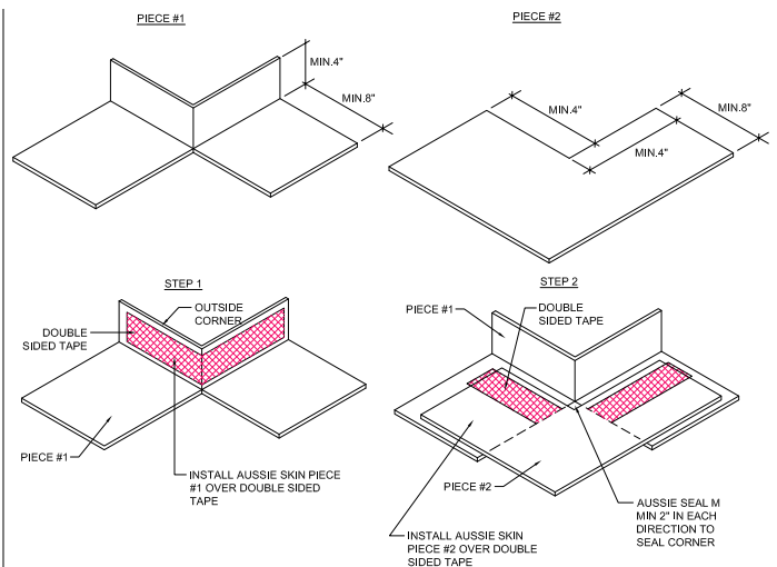
FIGURE 1.19 - OUTSIDE CORNER
