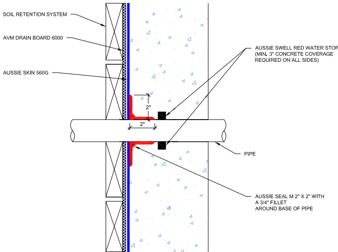
FIGURE 2.5 - PIPE PENETRATION THROUGH WALL
