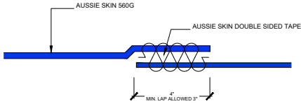
FIGURE 1.4 - DUAL SALVAGE EDGE FACTORY LAP
