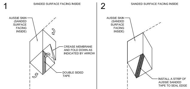
FIGURE 1.18 - INSIDE CORNER
