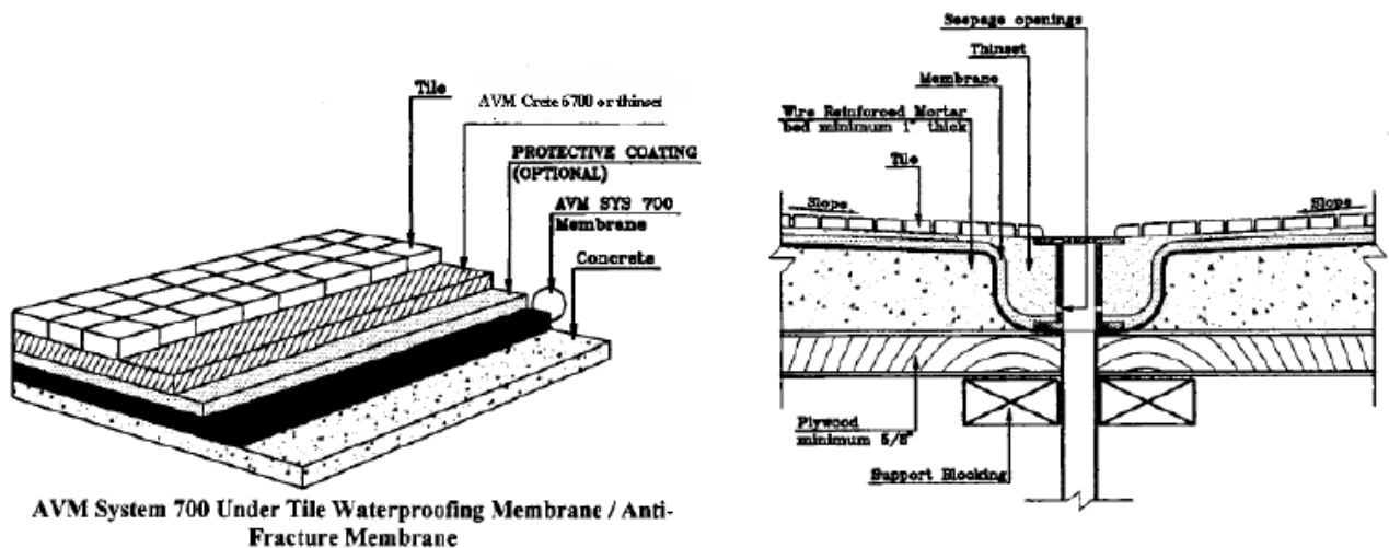
FIGURE 1—TYPICAL INSTALLATION DETAILS
