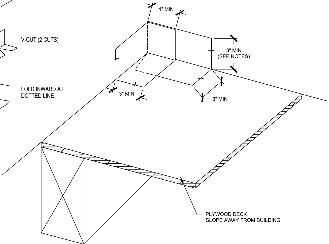
METAL FLASHING
